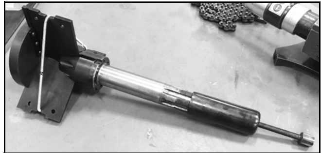
FIGURE 3-4. COMPLETED CENTER SHAFT SUB-ASSEMBLY
