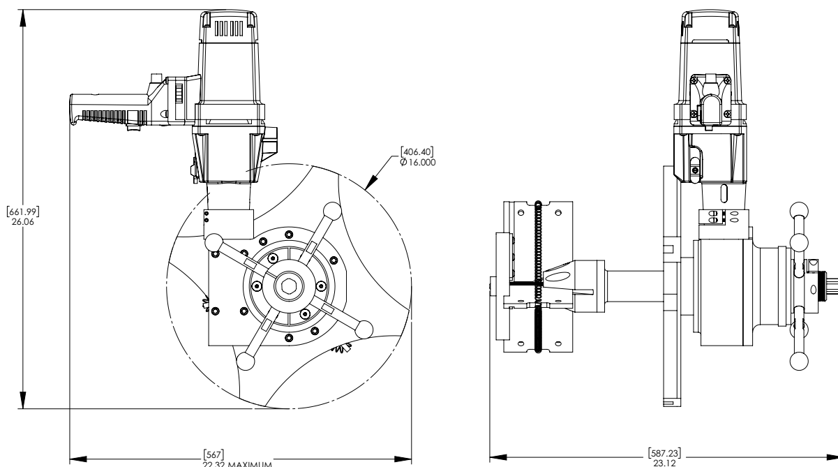
FIGURE 2-5. PB12 POWER BEVELER ELECTRIC DIMENSIONS (P/N PB12EL)
