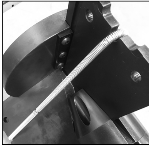
FIGURE 3-3. INSTALLATION OF THE WEDGE GUIDE ASSEMBLY
