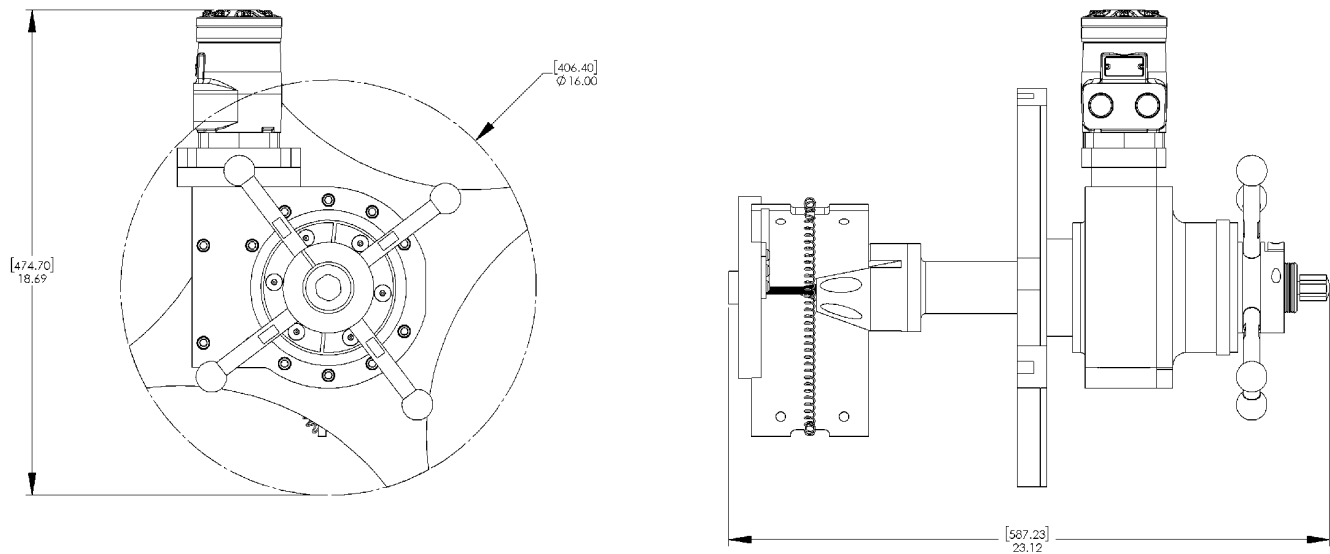
FIGURE 2-6. PB12 POWER BEVELER DIMENSIONS (P/N PB12HY)
