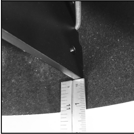
FIGURE 3-5. INSTALLED CENTER SHAFT ASSEMBLY
