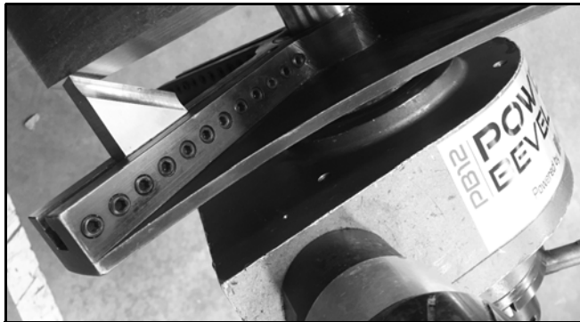
FIGURE 3-7. SINGLE CUTTING BIT INSTALLED
