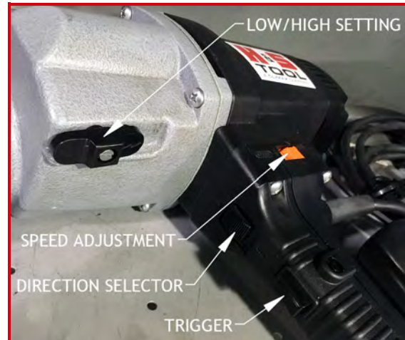
FIGURE 2-3. SPEED DIAL AND TRIGGER CONTROLS
