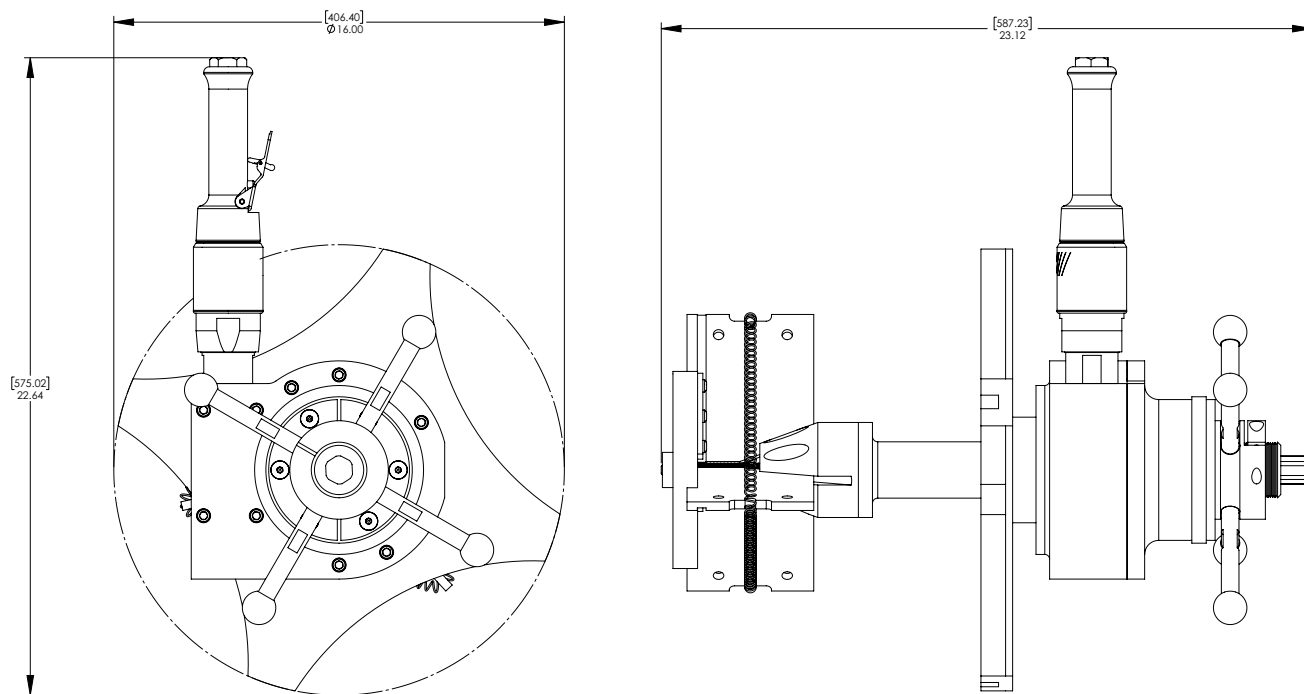
FIGURE 2-4. PB12 POWER BEVELER PNEUMATIC DIMENSIONS (P/N PB12PN)
