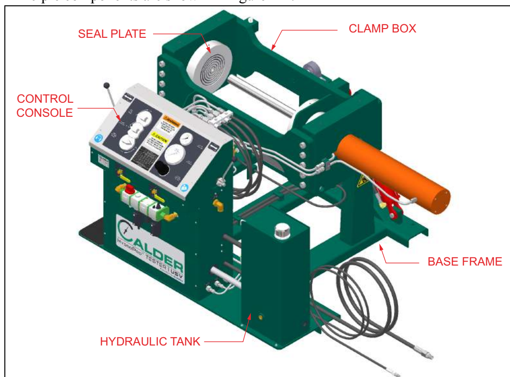
FIGURE 2-1. COMPONENTS
