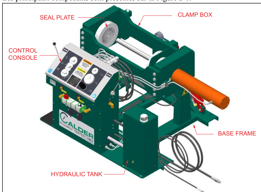
FIGURE 2-1. COMPOSANTS
