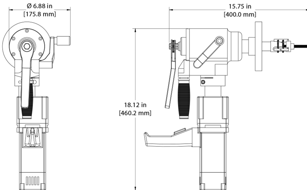
FIGURE 2-5. BG50 BOILER GUN ELECTRIC DIMENSIONS
