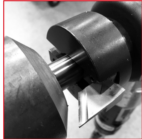
FIGURE 3-9. CUTTING BIT INSTALLED
