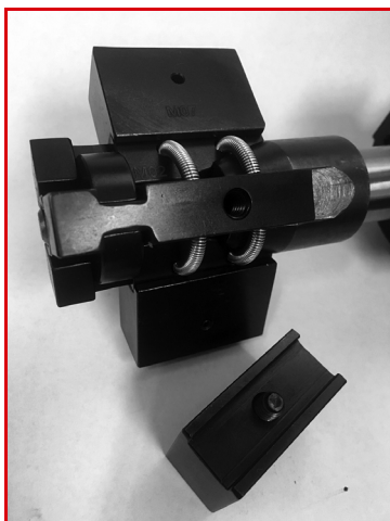
FIGURE 3-3. WEDGE EXTENSIONS INSTALLATION
