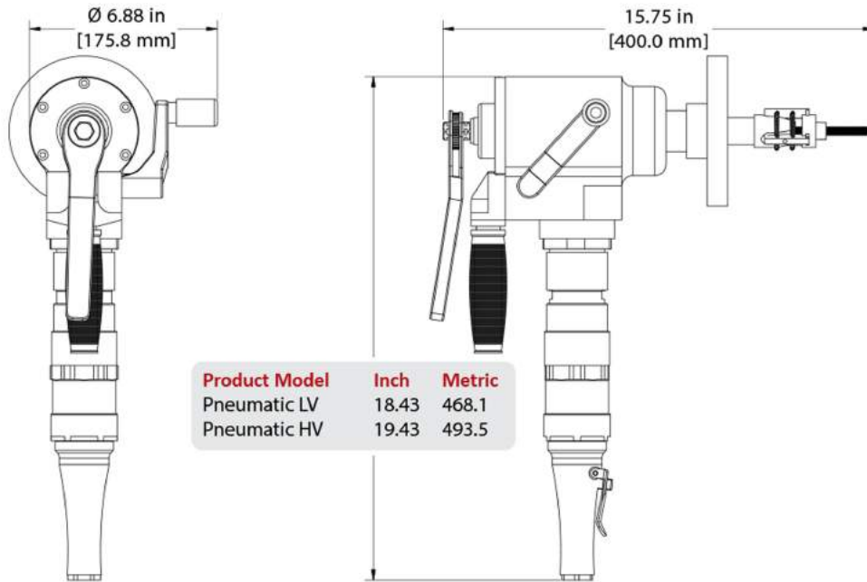
FIGURE 2-4. BG50 BOILER GUN PNEUMATIC DIMENSIONS
