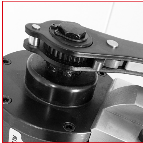
FIGURE 3-7. LOCKING ROD WRENCH WITH SPEED WHEEL
