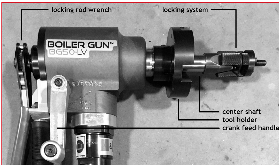
FIGURE 3-1. BG50 BOILER GUN MAIN COMPONENTS
