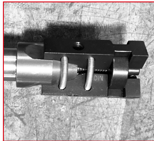
FIGURE 3-2. INSTALLED WEDGE SET
