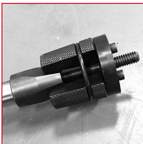
FIGURE 3-4. THE 1.25" COLLET SET INSTALLED
