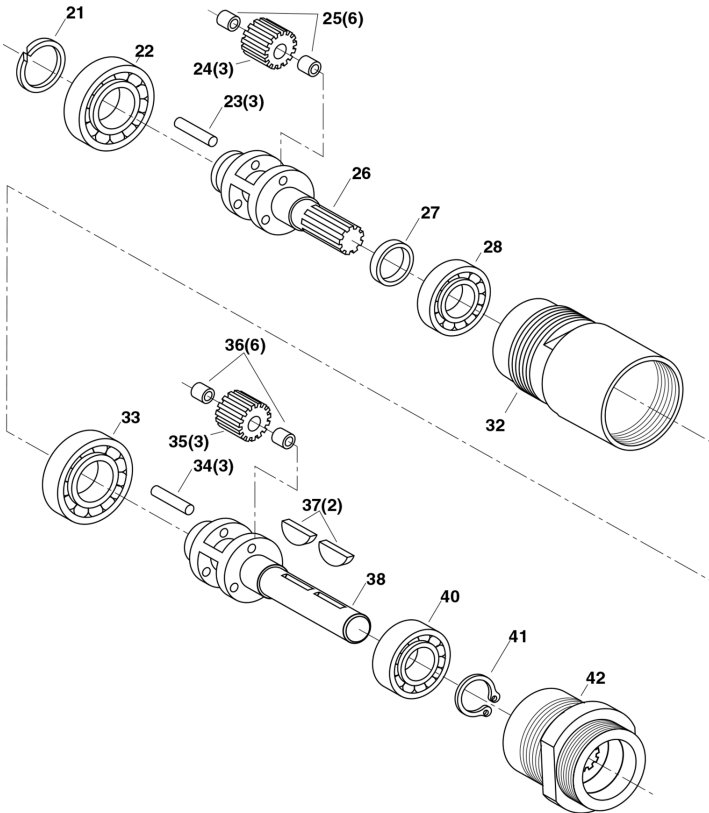
FIGURE A-10. LV AIR MOTOR ASSEMBLY AND PARTS LIST (P/N CML3488)
