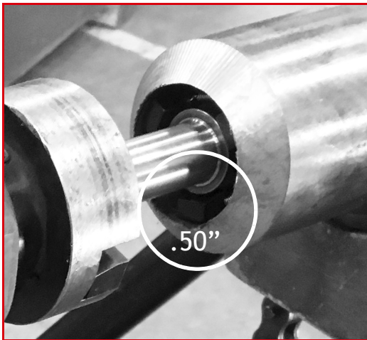
FIGURE 3-6. BG50 INSTALLED IN WORKPIECE
