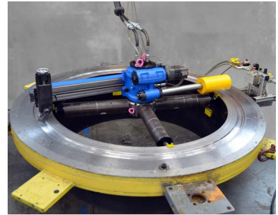
FF6300 Flange Facer
