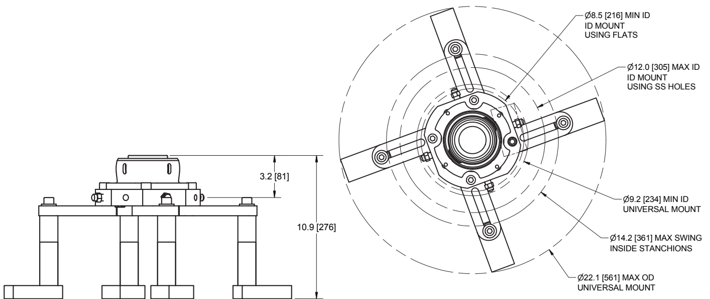
Spherical bearing mount assembly
