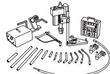
BW3000 Auto Bore Welder
